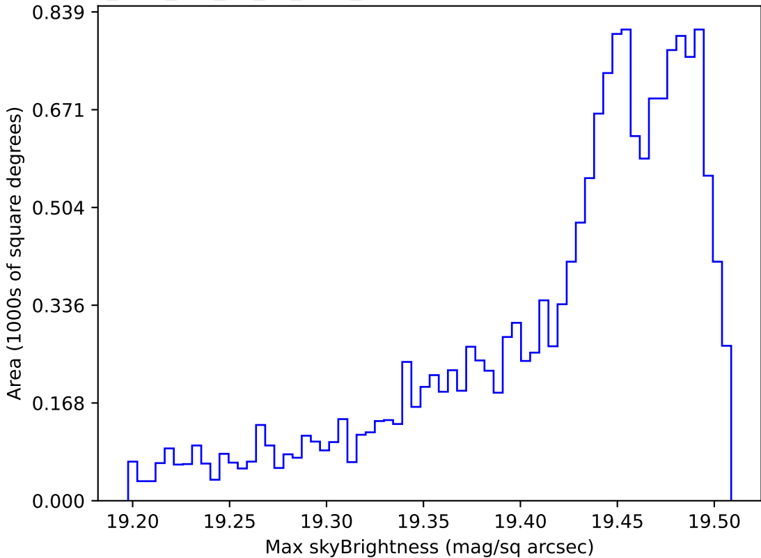
too_elab_r32_d3_gz_v3.4_10yrs WFD z band: Max skyBrightness
