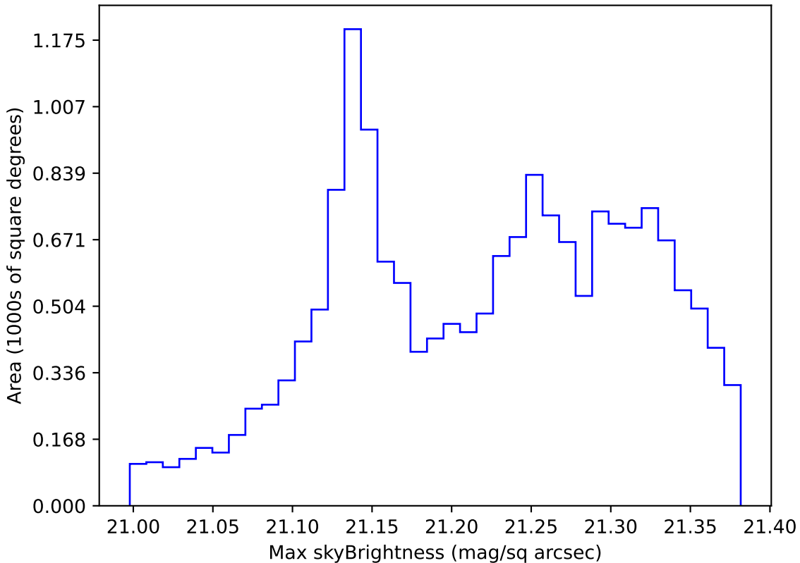
too_elab_r32_d3_gz_v3.4_10yrs WFD r band: Max skyBrightness
