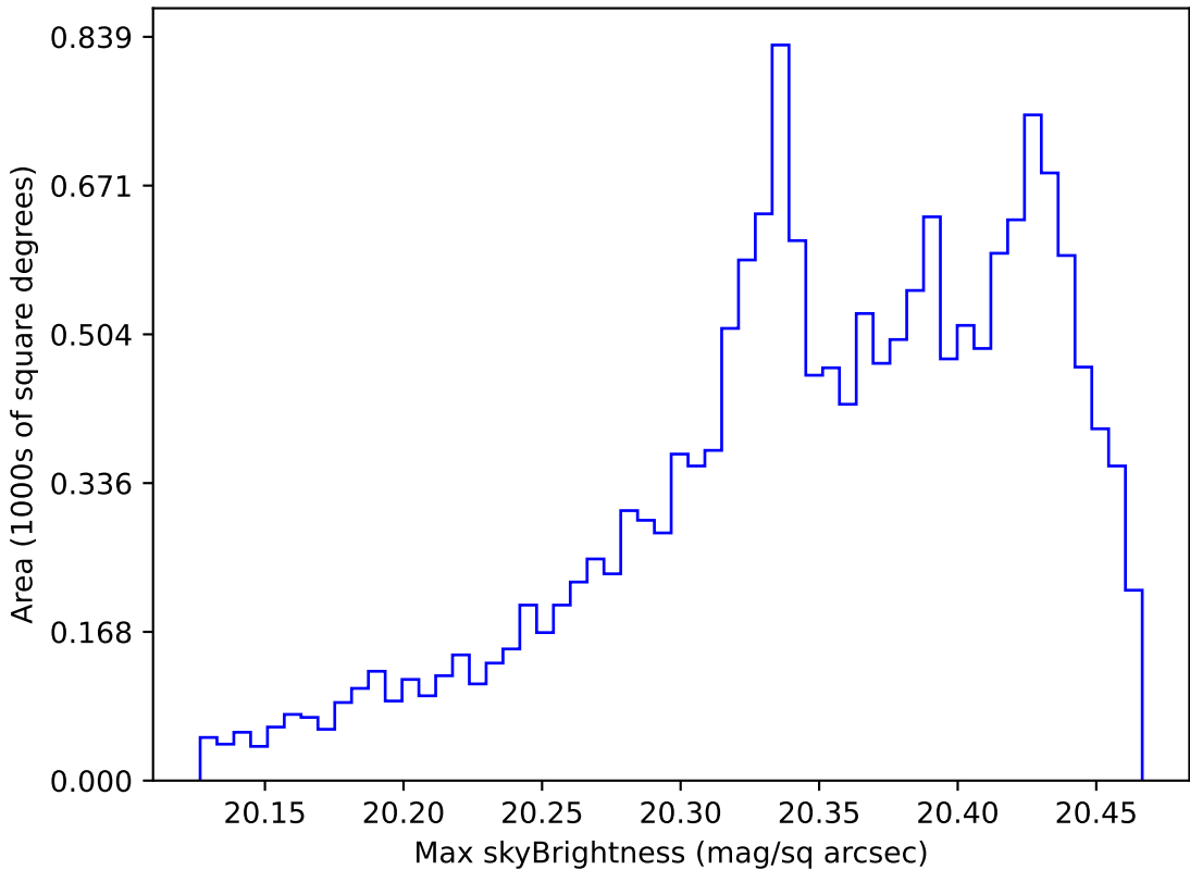
too_elab_r32_d3_gz_v3.4_10yrs WFD i band: Max skyBrightness
