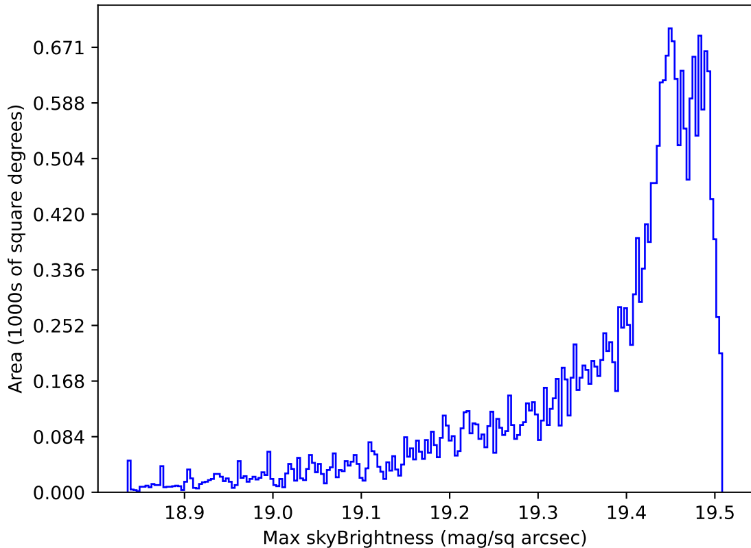
too_elab_r32_d3_gz_v3.4_10yrs All sky z band: Max skyBrightness
