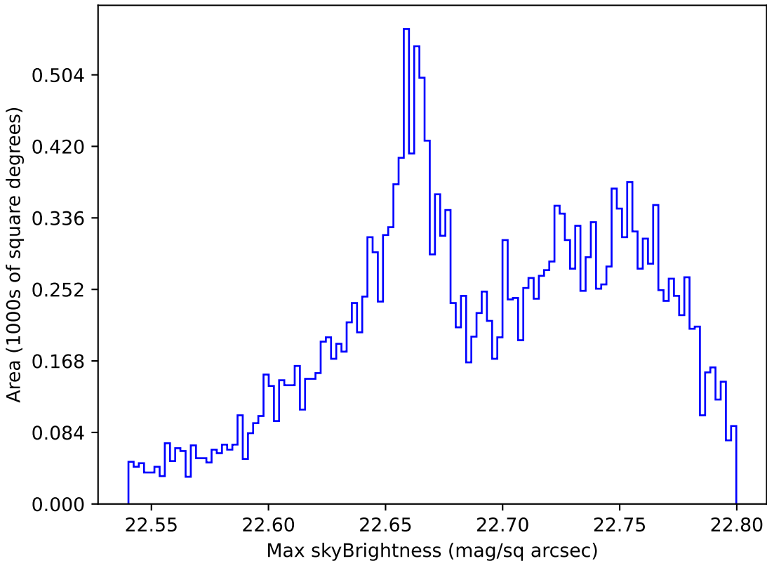
too_elab_r32_d3_gz_v3.4_10yrs All sky u band: Max skyBrightness
