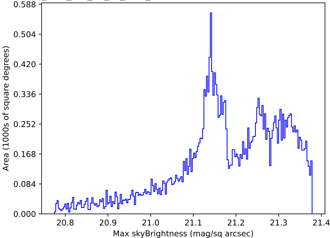
too_elab_r32_d3_gz_v3.4_10yrs All sky r band: Max skyBrightness
