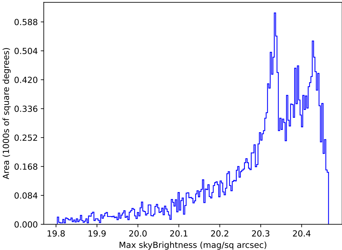
too_elab_r32_d3_gz_v3.4_10yrs All sky i band: Max skyBrightness
