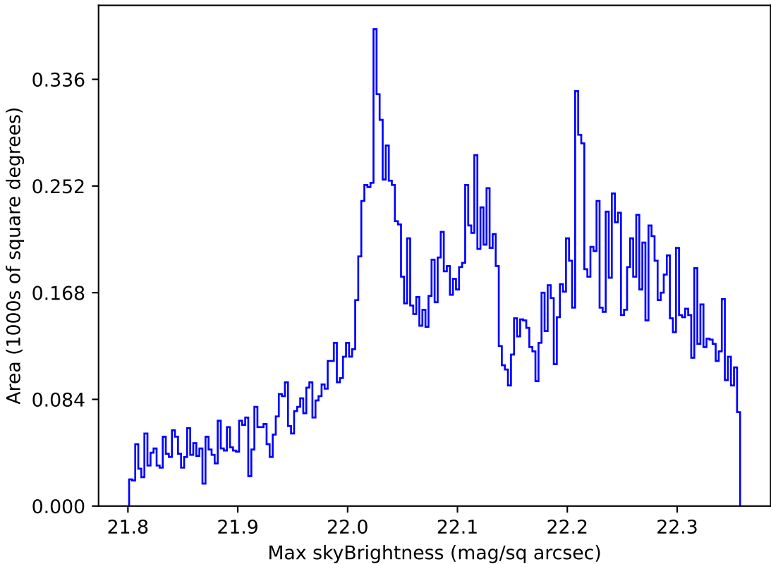
too_elab_r32_d3_gz_v3.4_10yrs All sky g band: Max skyBrightness
