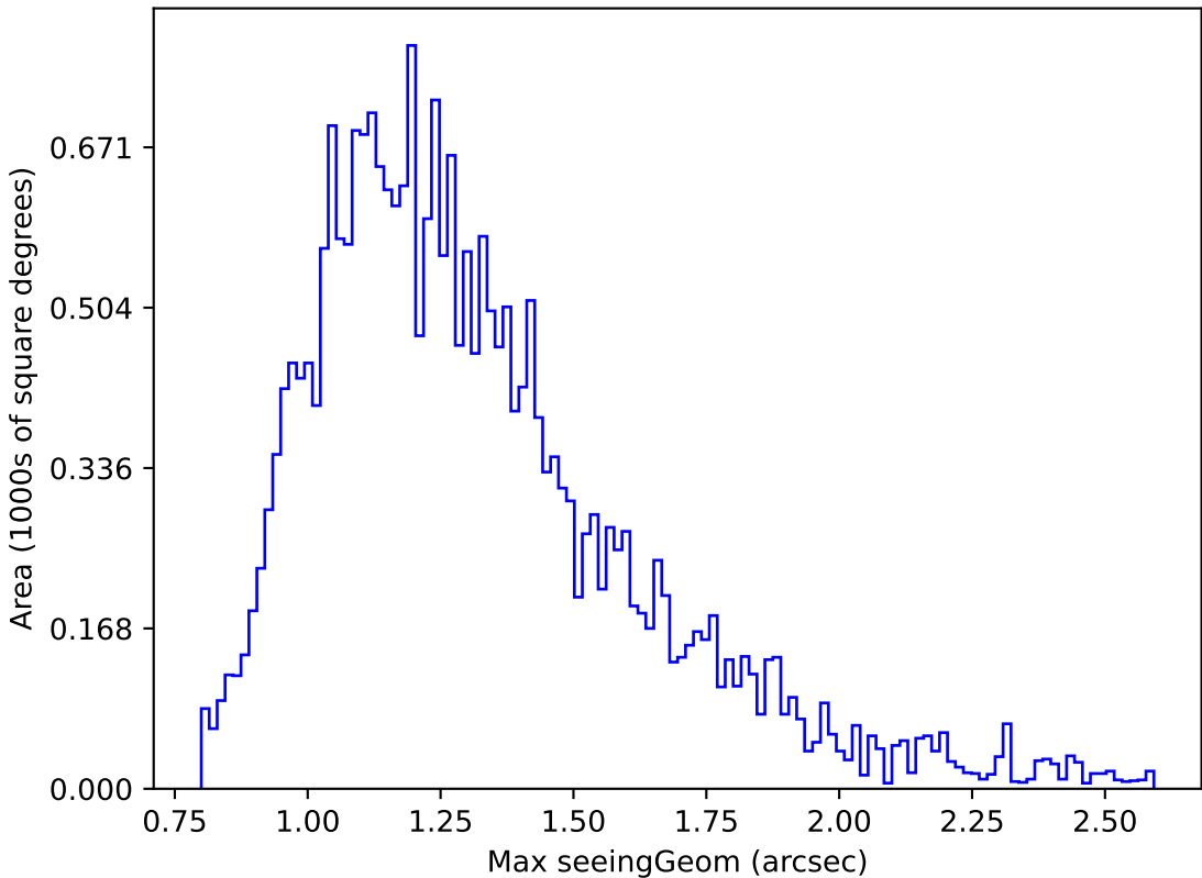
too_elab_r32_d3_gz_v3.4_10yrs Yr 1 z band: Max seeingGeom
