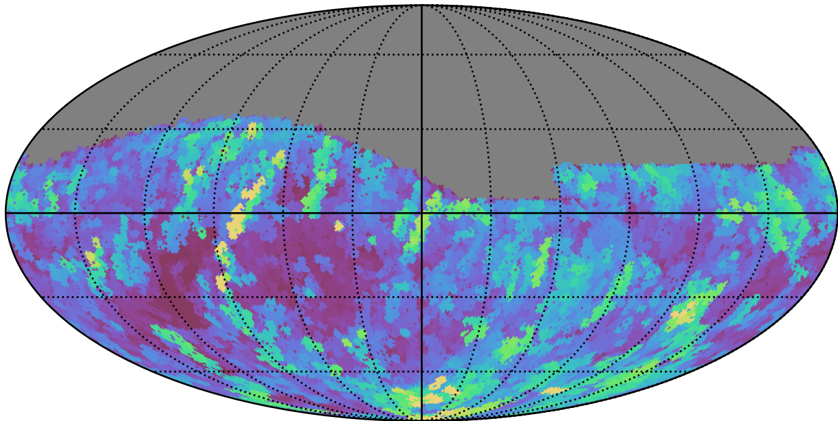
too_elab_r32_d3_gz_v3.4_10yrs Yr 1 r band: Max seeingGeom
