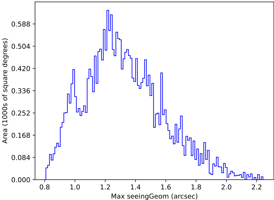
too_elab_r32_d3_gz_v3.4_10yrs Yr 1 r band: Max seeingGeom
