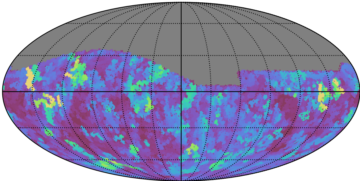
too_elab_r32_d3_gz_v3.4_10yrs Yr 1 i band: Max seeingGeom
