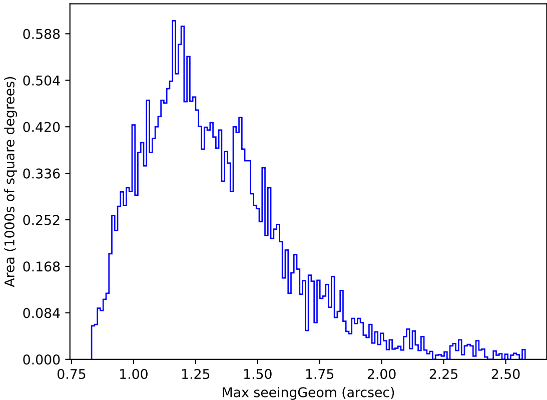
too_elab_r32_d3_gz_v3.4_10yrs Yr 1 i band: Max seeingGeom
