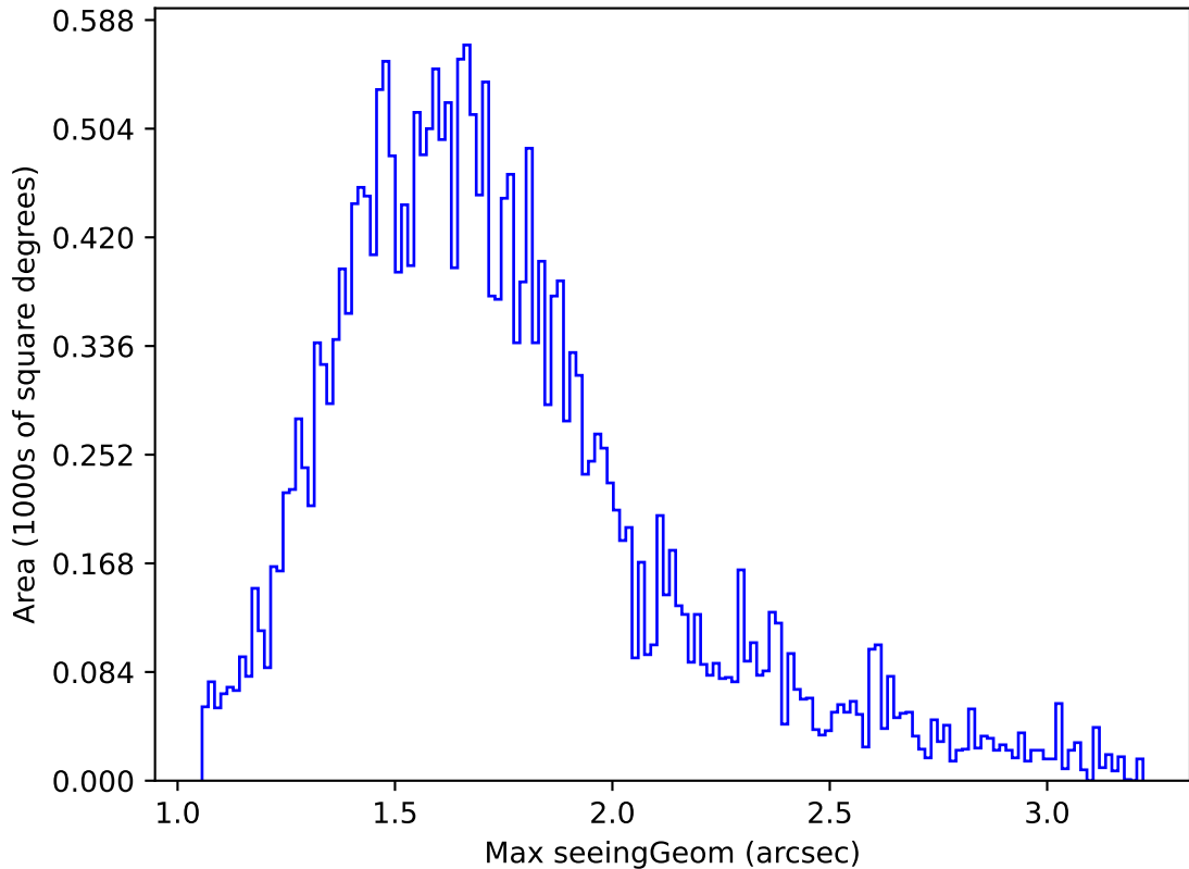
too_elab_r32_d3_gz_v3.4_10yrs Yr 1 all bands: Max seeingGeom
