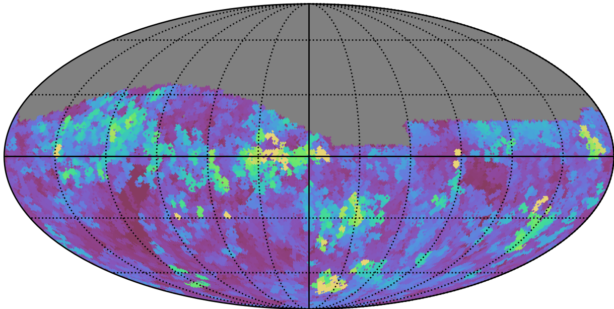
too_elab_r32_d3_gz_v3.4_10yrs Yr 1 z band: Max seeingEff
