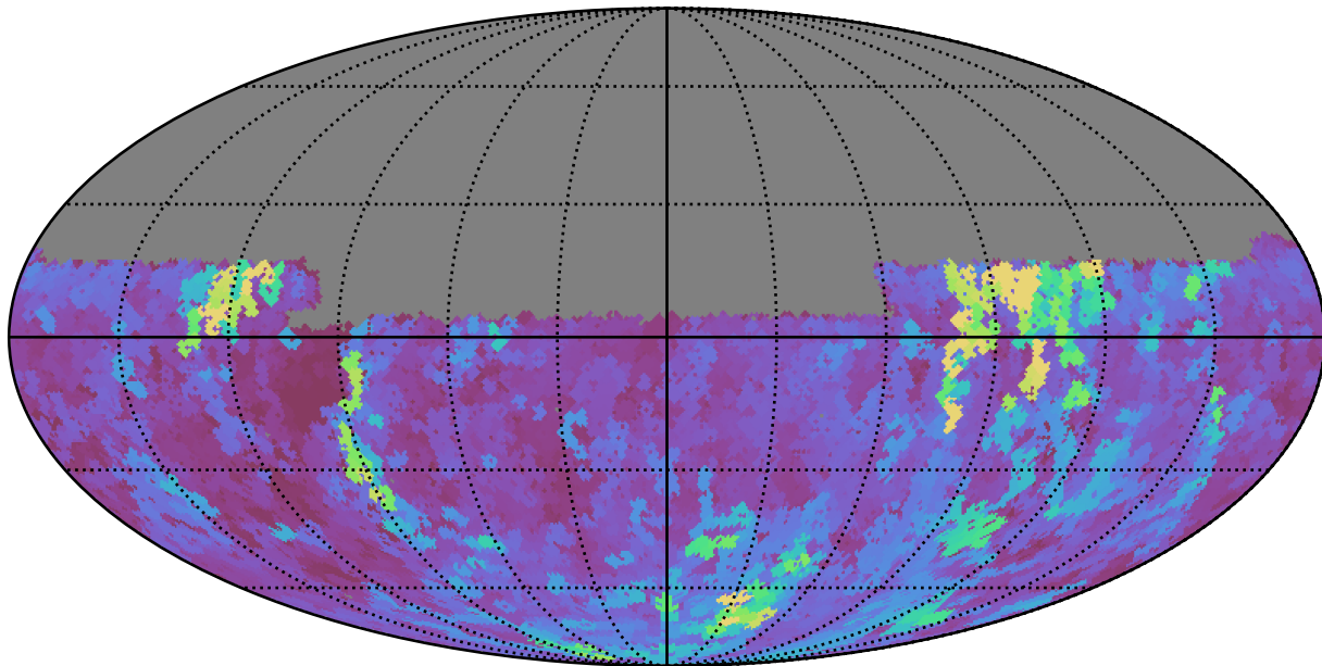
too_elab_r32_d3_gz_v3.4_10yrs Yr 1 u band: Max seeingEff
