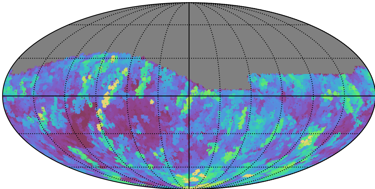
too_elab_r32_d3_gz_v3.4_10yrs Yr 1 r band: Max seeingEff
