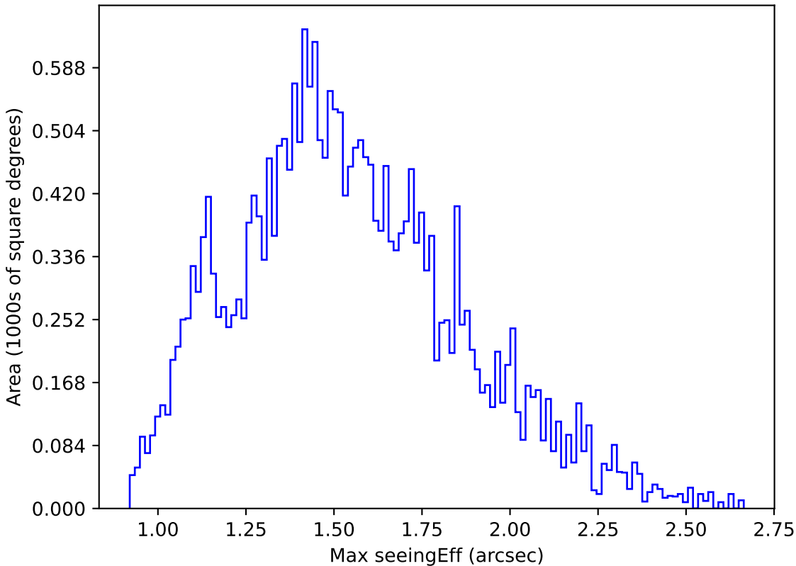
too_elab_r32_d3_gz_v3.4_10yrs Yr 1 r band: Max seeingEff
