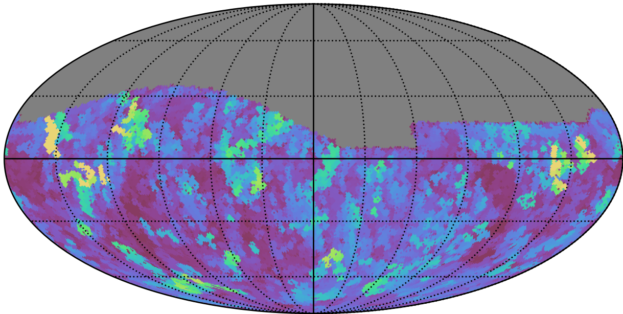
too_elab_r32_d3_gz_v3.4_10yrs Yr 1 i band: Max seeingEff
