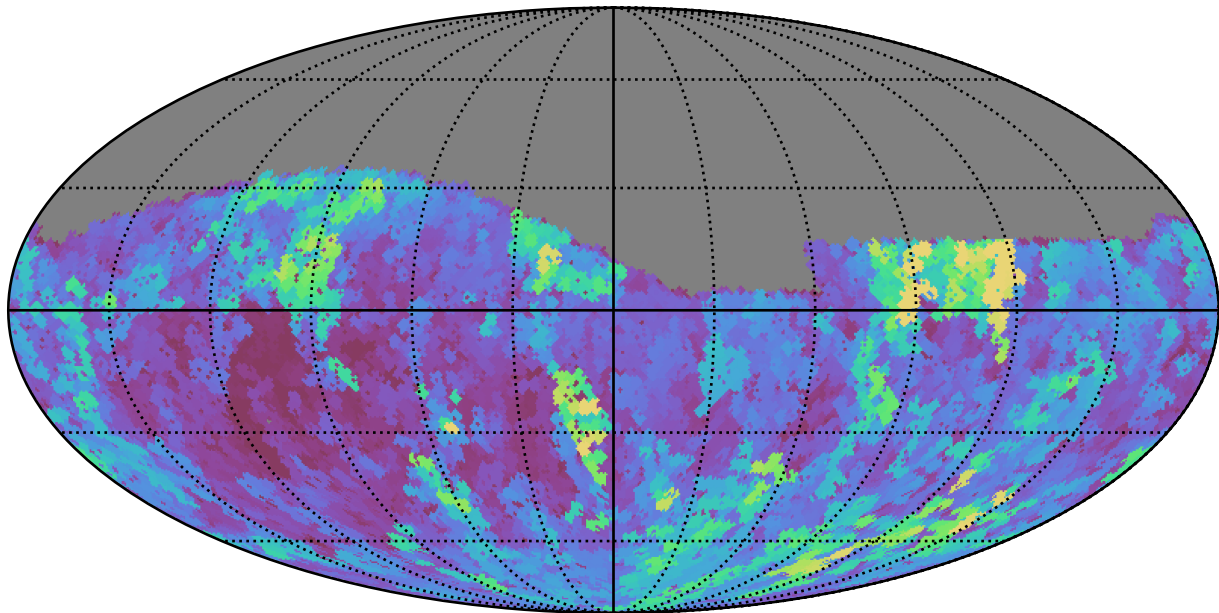
too_elab_r32_d3_gz_v3.4_10yrs Yr 1 g band: Max seeingEff
