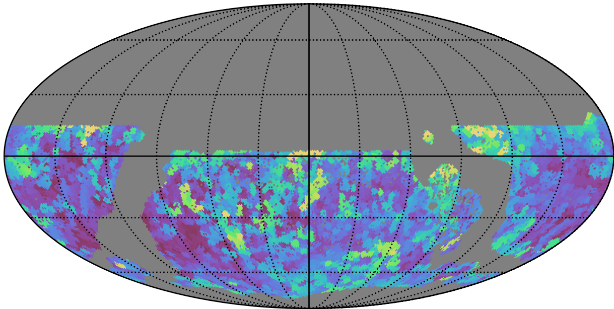
too_elab_r32_d3_gz_v3.4_10yrs WFD r band: Max seeingEff
