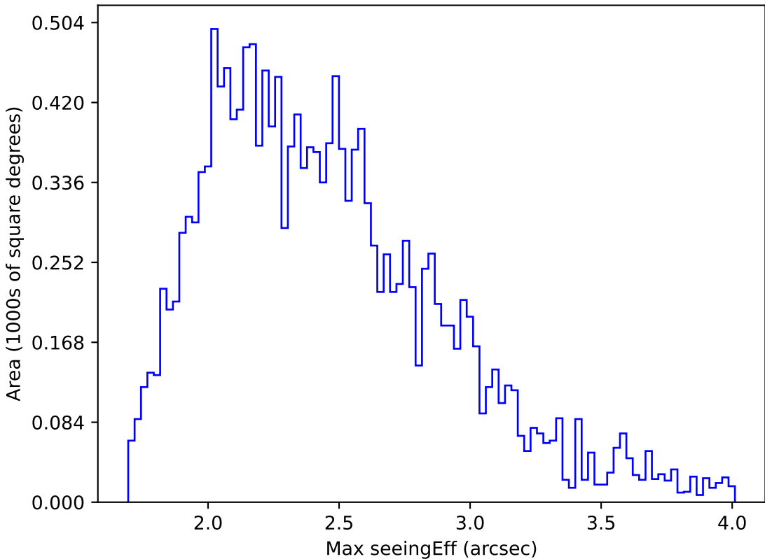
too_elab_r32_d3_gz_v3.4_10yrs WFD g band: Max seeingEff
