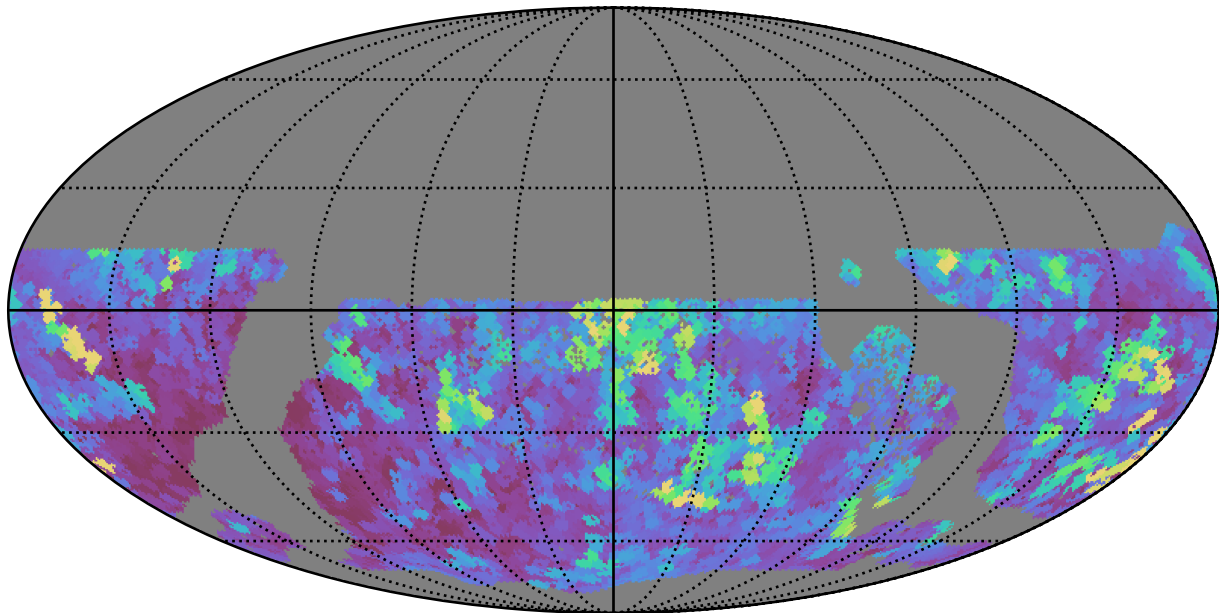
too_elab_r32_d3_gz_v3.4_10yrs WFD all bands: Max seeingEff
