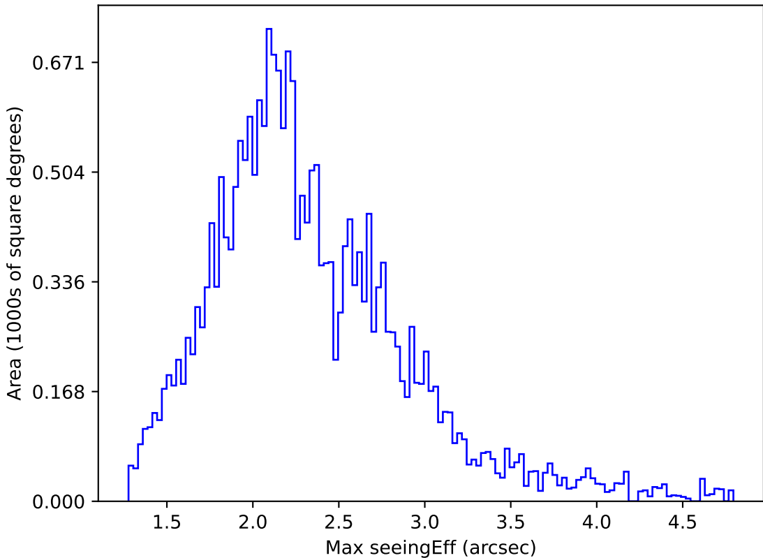
too_elab_r32_d3_gz_v3.4_10yrs All sky y band: Max seeingEff
