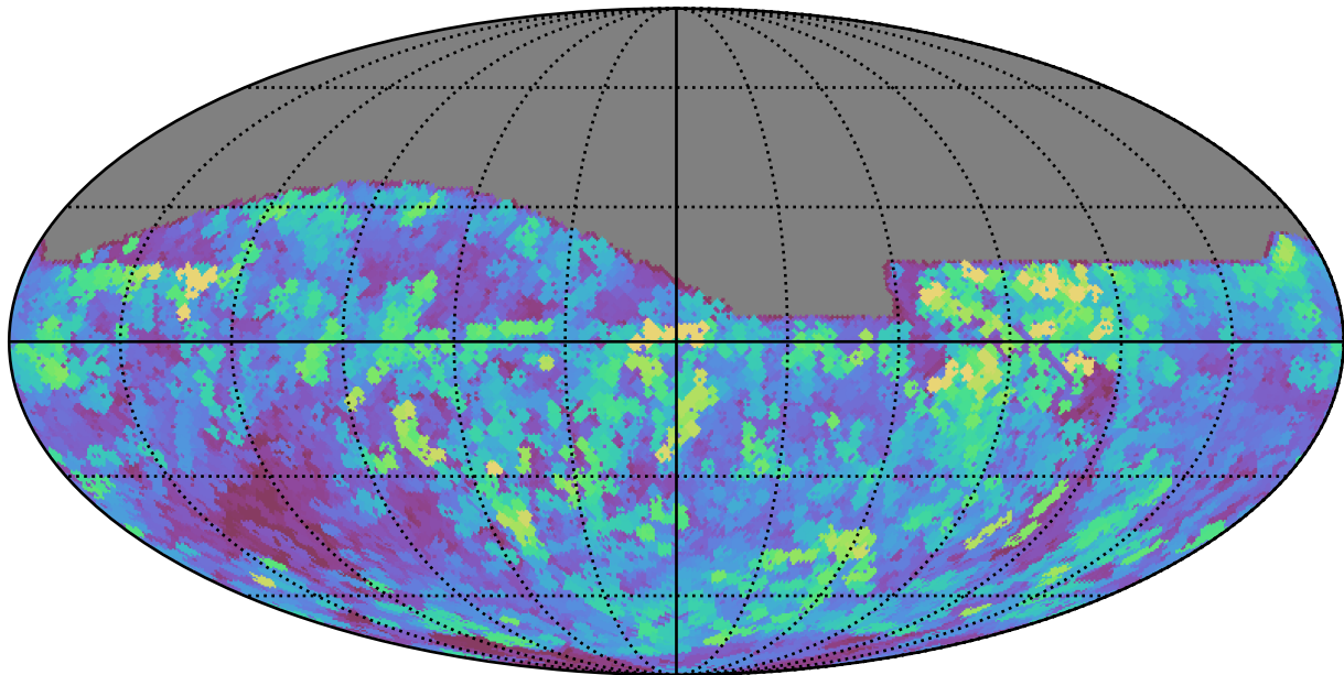
too_elab_r32_d3_gz_v3.4_10yrs All sky r band: Max seeingEff
