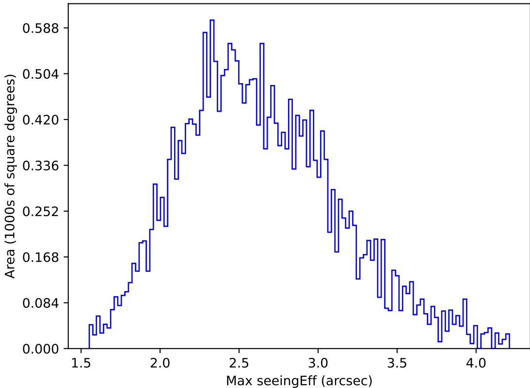
too_elab_r32_d3_gz_v3.4_10yrs All sky r band: Max seeingEff
