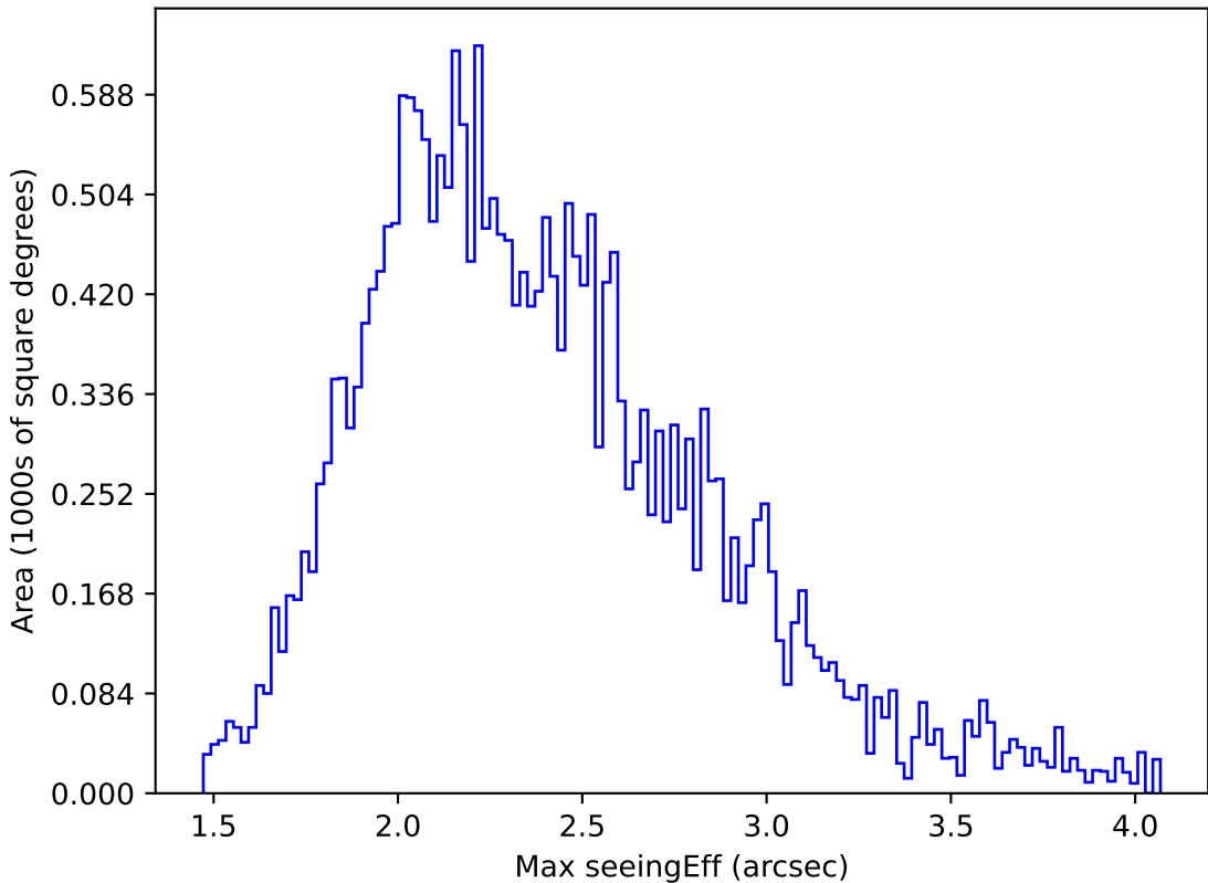
too_elab_r32_d3_gz_v3.4_10yrs All sky g band: Max seeingEff
