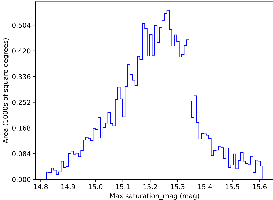
too_elab_r32_d3_gz_v3.4_10yrs WFD z band: Max saturation_mag
