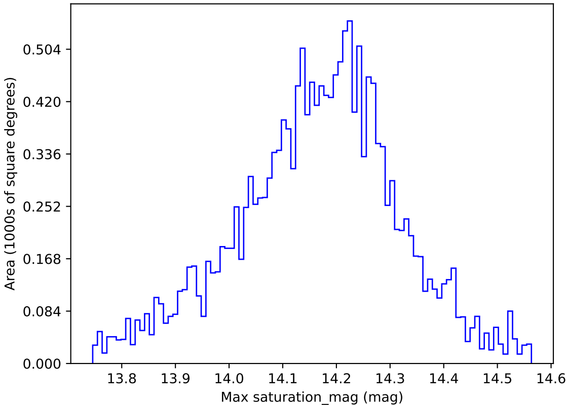
too_elab_r32_d3_gz_v3.4_10yrs WFD y band: Max saturation_mag
