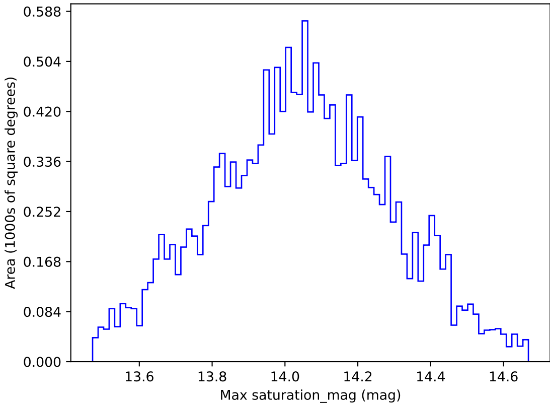
too_elab_r32_d3_gz_v3.4_10yrs WFD u band: Max saturation_mag
