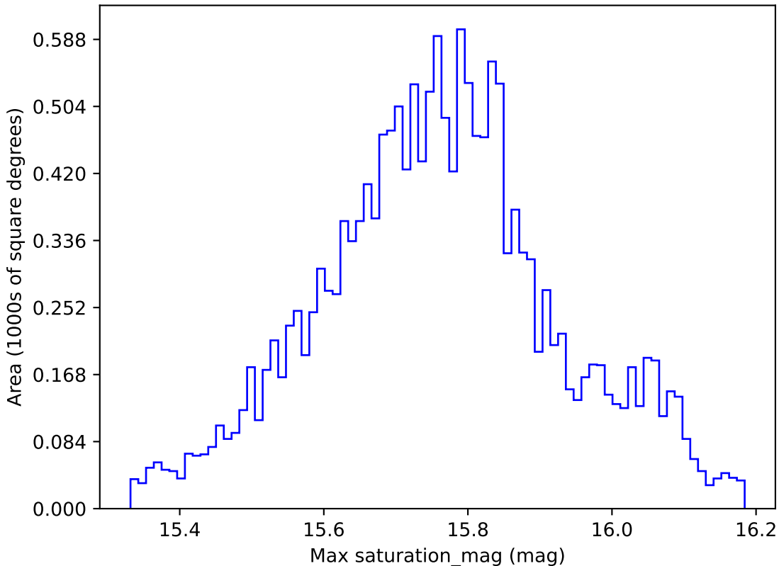
too_elab_r32_d3_gz_v3.4_10yrs WFD r band: Max saturation_mag
