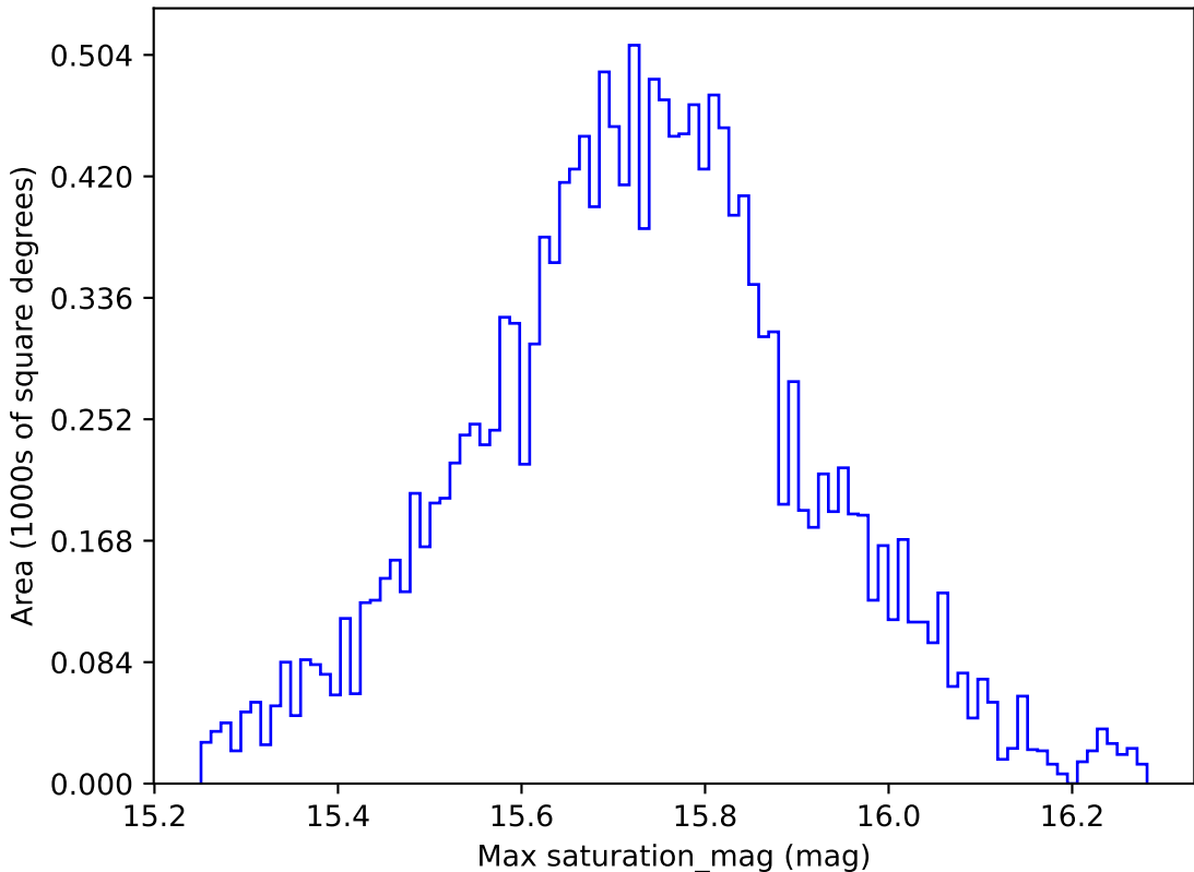
too_elab_r32_d3_gz_v3.4_10yrs WFD g band: Max saturation_mag
