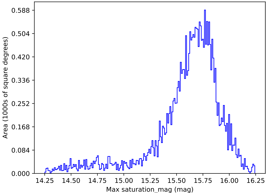
too_elab_r32_d3_gz_v3.4_10yrs All sky g band: Max saturation_mag
