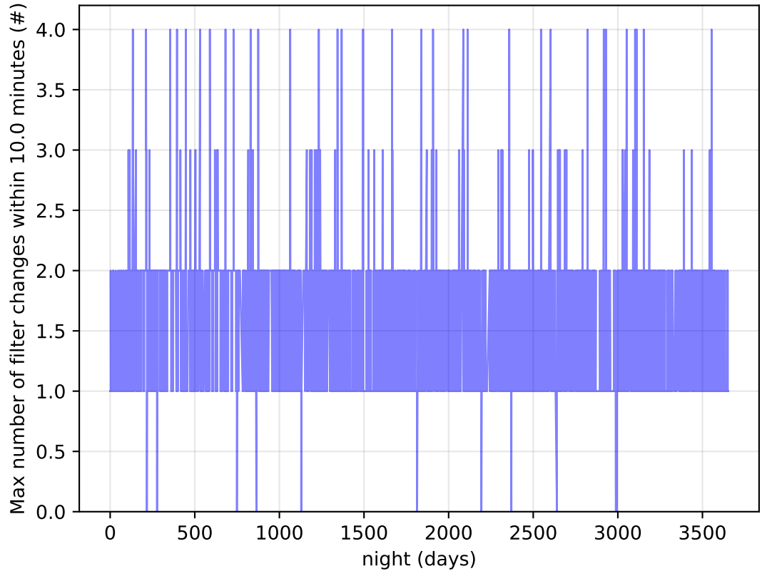
too_elab_r32_d3_gz_v3.4_10yrs Per Night: Max number of filter changes within 10.0 minutes
