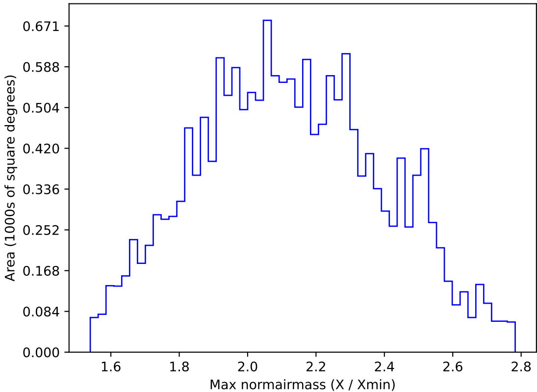
too_elab_r32_d3_gz_v3.4_10yrs WFD y band: Max normairmass
