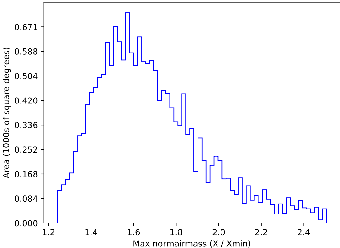
too_elab_r32_d3_gz_v3.4_10yrs WFD u band: Max normairmass
