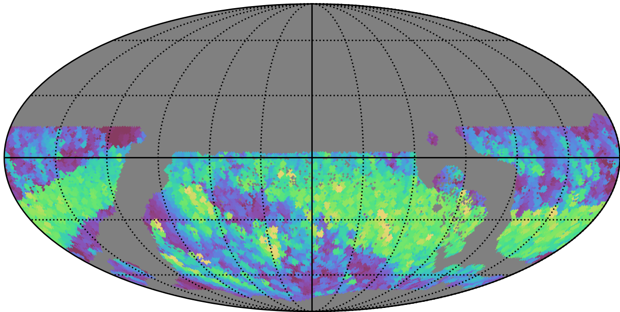
too_elab_r32_d3_gz_v3.4_10yrs WFD r band: Max normairmass
