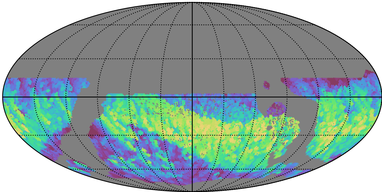
too_elab_r32_d3_gz_v3.4_10yrs WFD i band: Max normairmass
