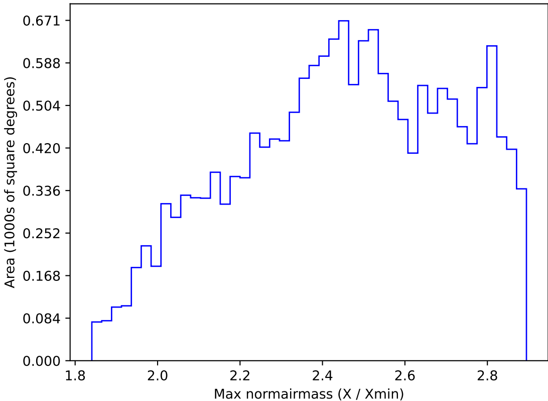
too_elab_r32_d3_gz_v3.4_10yrs WFD all bands: Max normairmass
