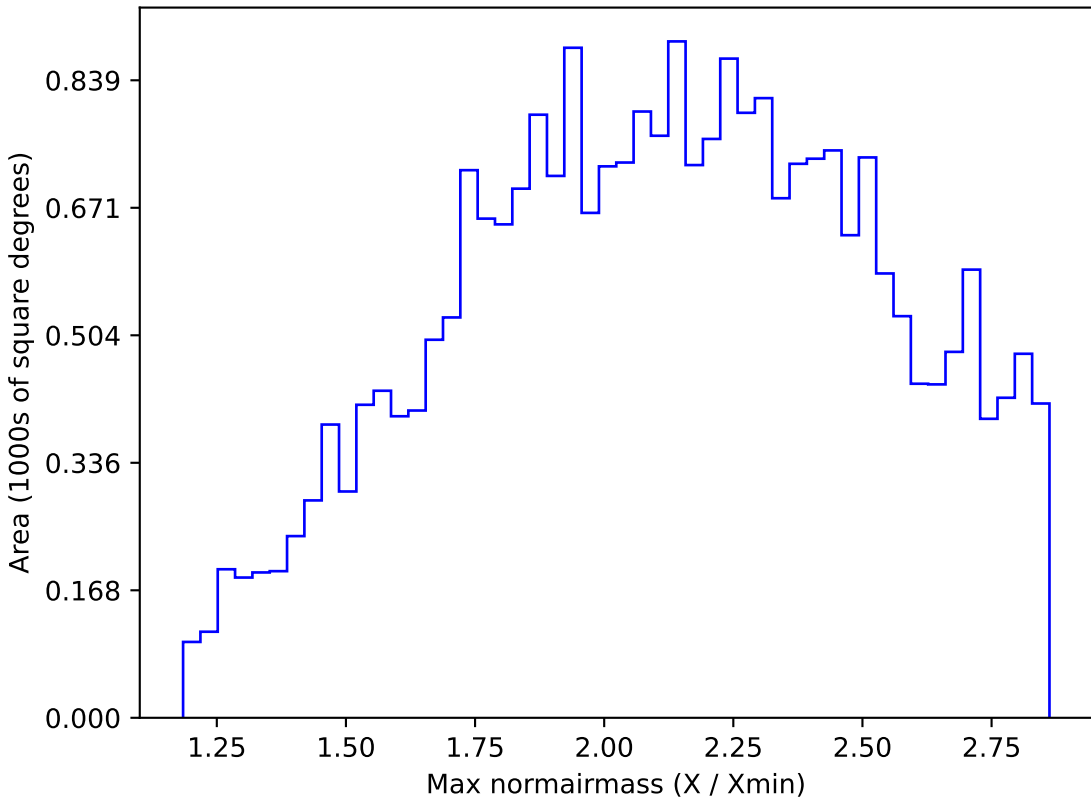
too_elab_r32_d3_gz_v3.4_10yrs All sky z band: Max normairmass
