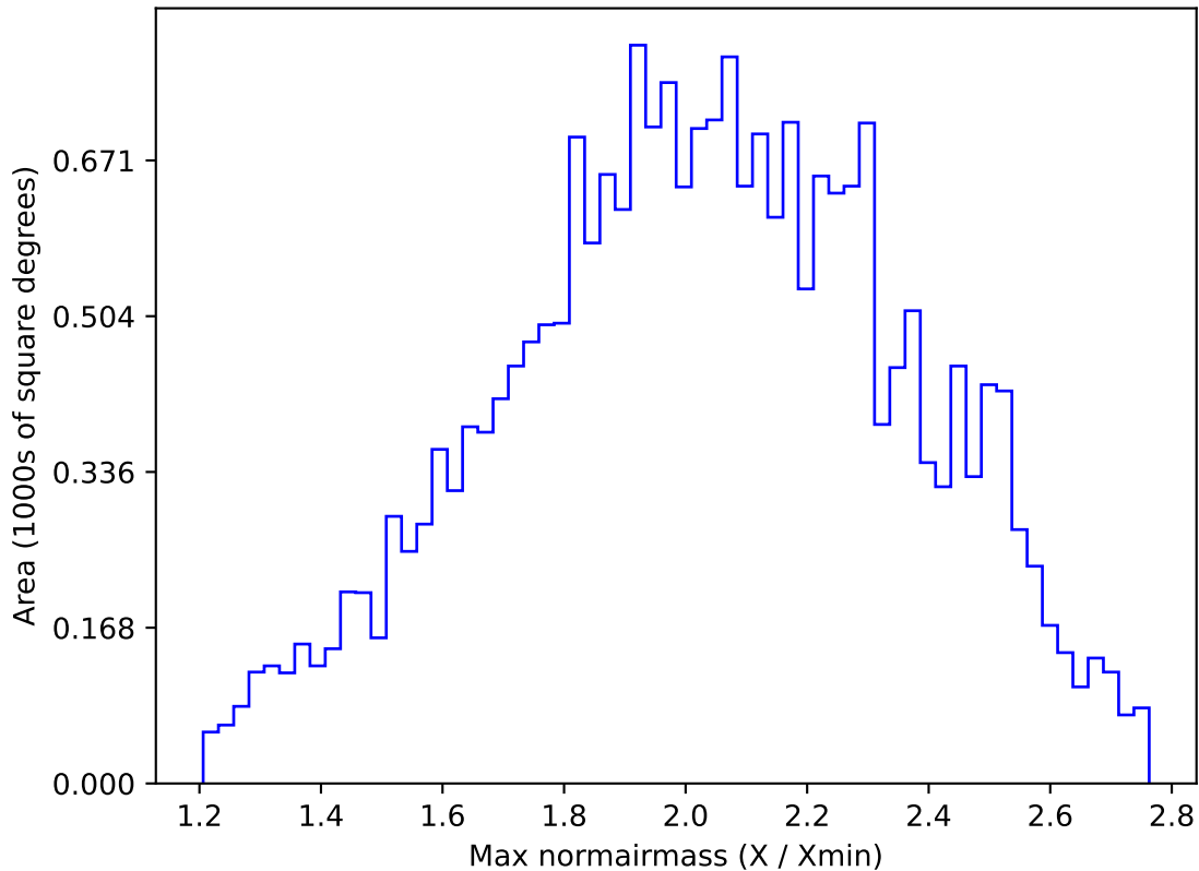
too_elab_r32_d3_gz_v3.4_10yrs All sky y band: Max normairmass
