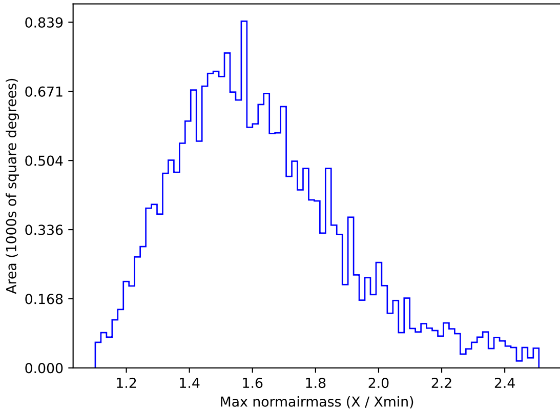
too_elab_r32_d3_gz_v3.4_10yrs All sky u band: Max normairmass
