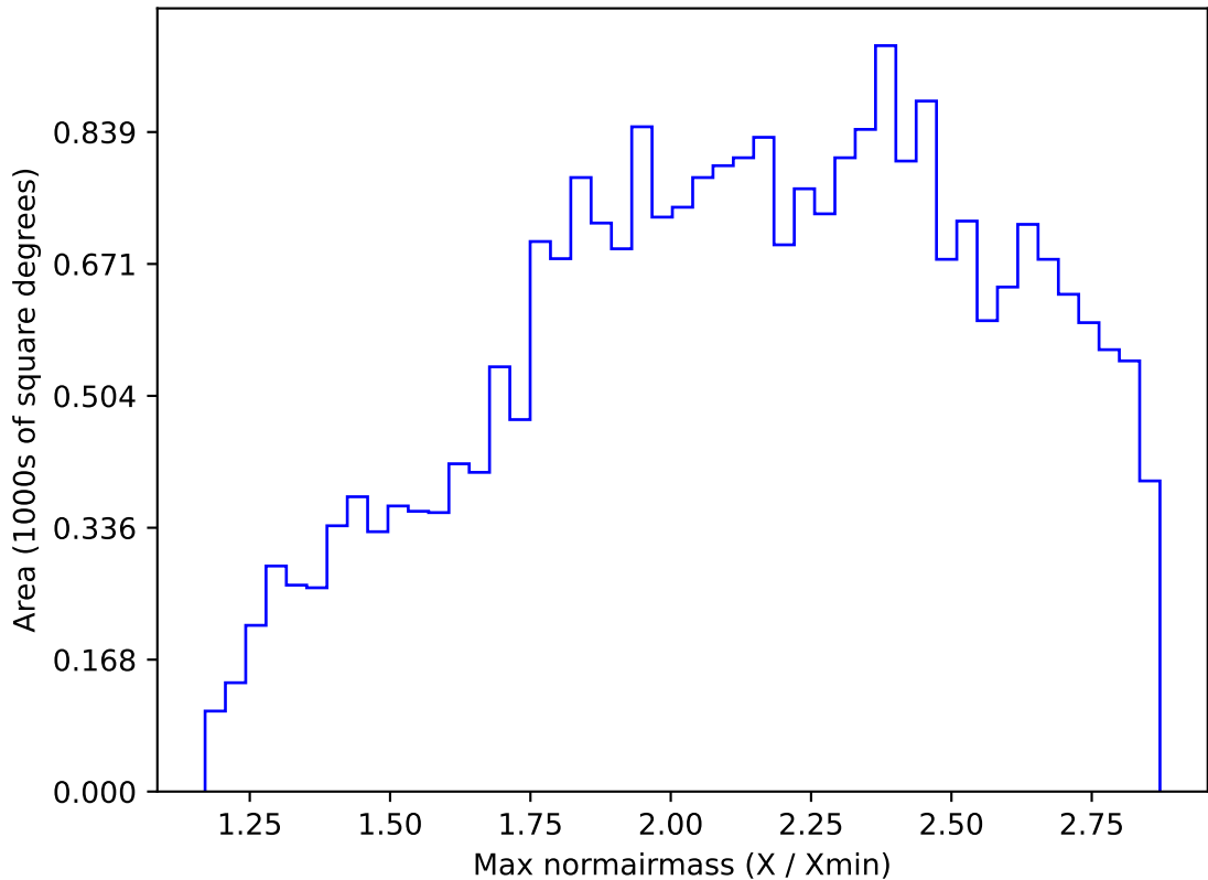
too_elab_r32_d3_gz_v3.4_10yrs All sky i band: Max normairmass
