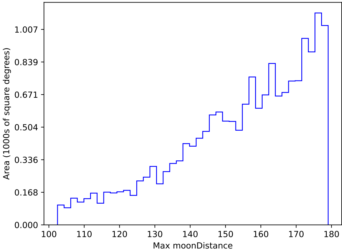
too_elab_r32_d3_gz_v3.4_10yrs WFD z band: Max moonDistance
