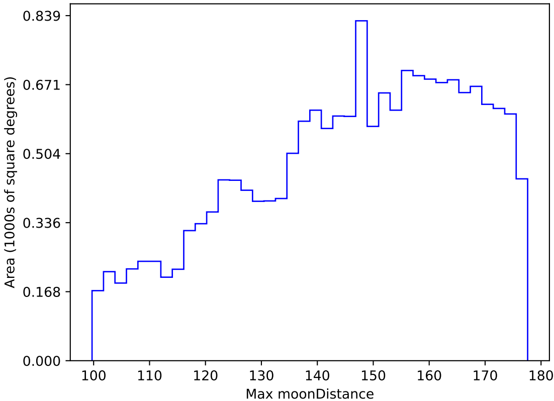
too_elab_r32_d3_gz_v3.4_10yrs WFD y band: Max moonDistance
