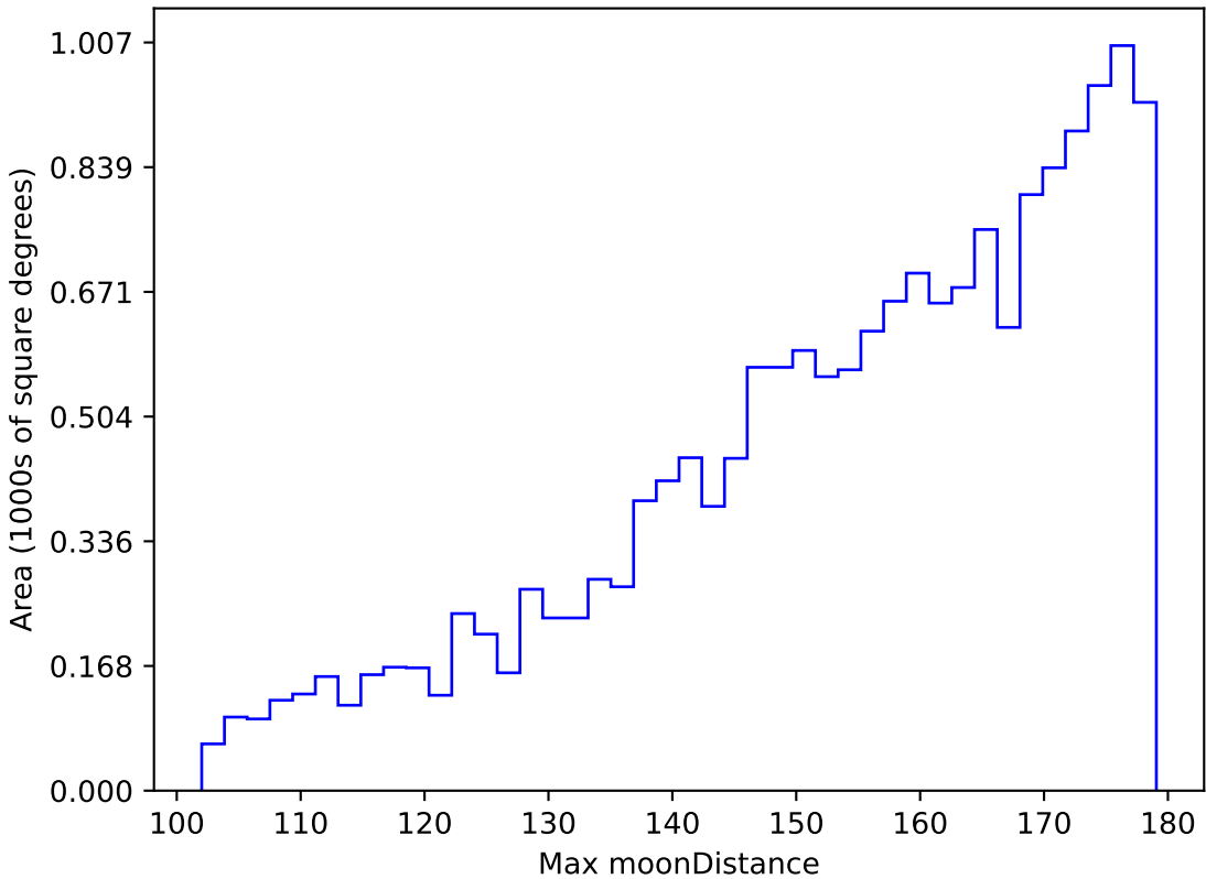
too_elab_r32_d3_gz_v3.4_10yrs WFD u band: Max moonDistance
