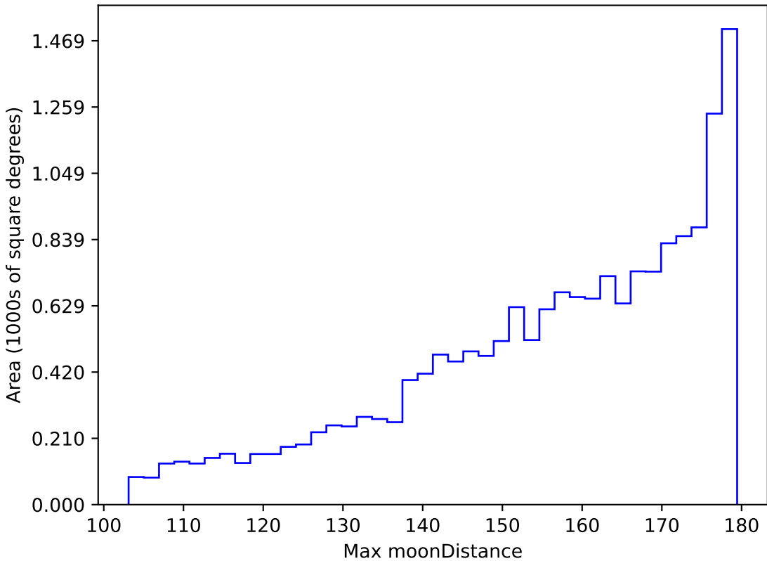
too_elab_r32_d3_gz_v3.4_10yrs WFD r band: Max moonDistance
