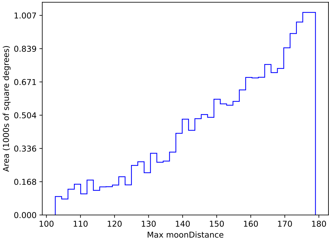
too_elab_r32_d3_gz_v3.4_10yrs WFD g band: Max moonDistance
