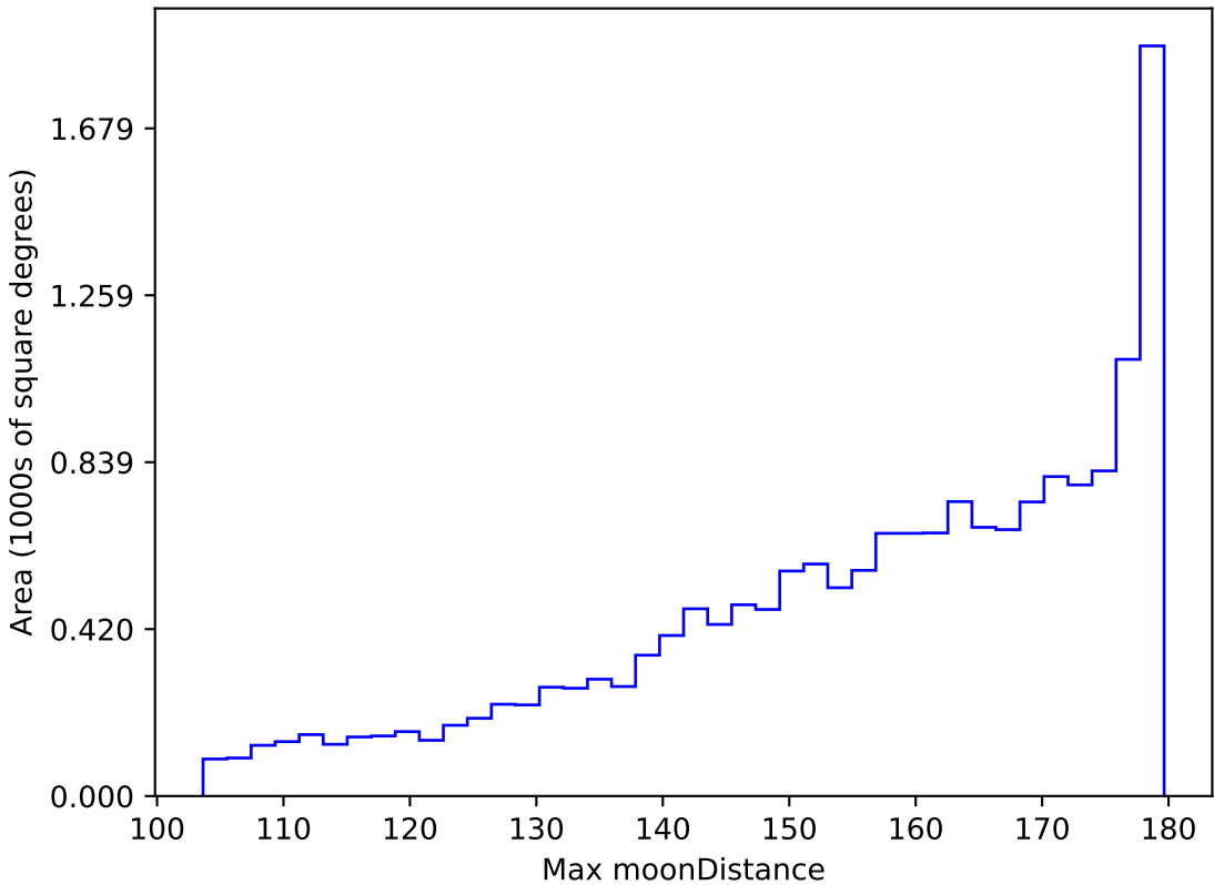
too_elab_r32_d3_gz_v3.4_10yrs WFD all bands: Max moonDistance
