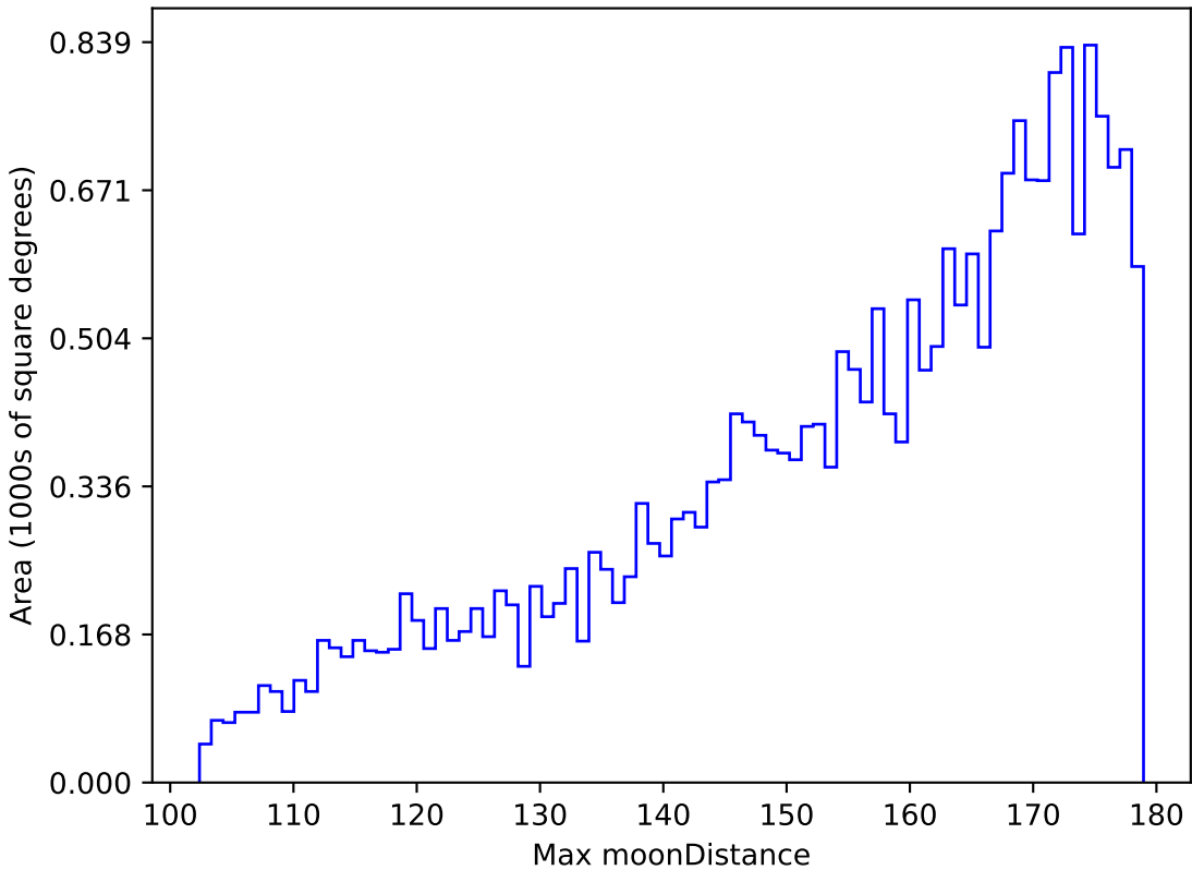
too_elab_r32_d3_gz_v3.4_10yrs All sky z band: Max moonDistance
